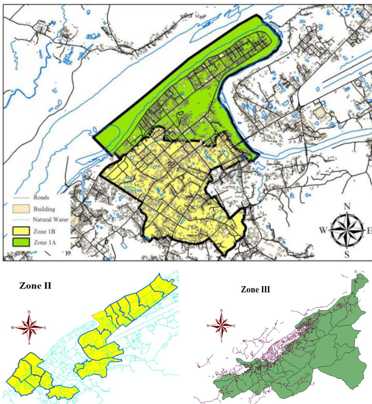
Figure 20. Luang Prabang City drainage zones (UDAA 2013)
