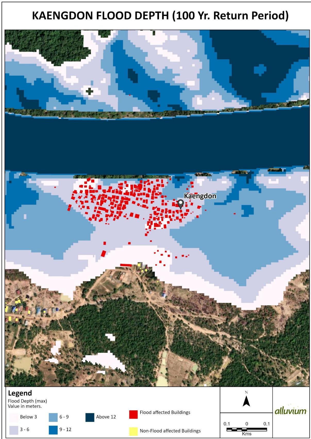
Figure 16. Flood extent and depth for storm event with a 100-year return period (current climate) for Kaengdon Village
