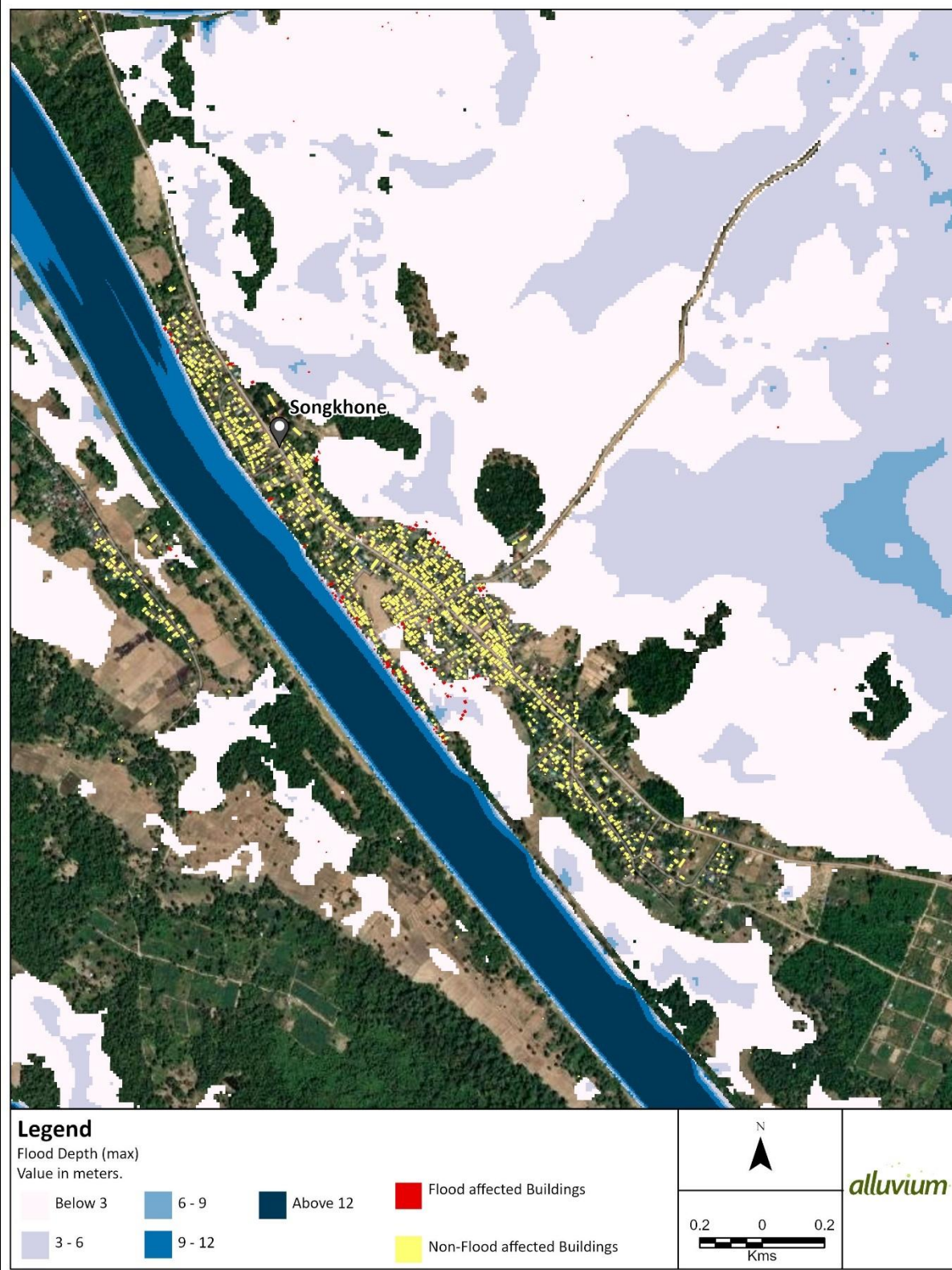
Figure 17. Flood extent and depth for storm event with a 10-year return period (current climate) for Songkhone Village
