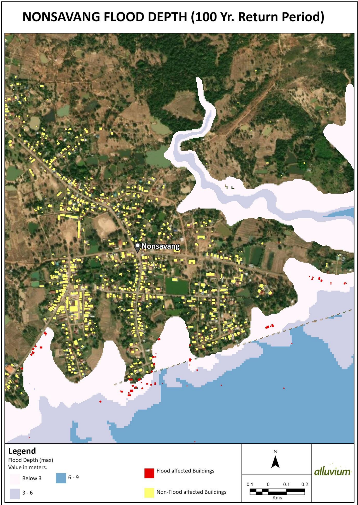
Figure 16. Flood extent and depth for storm event with a 100-year return period (current climate) for Nonsavang Village
