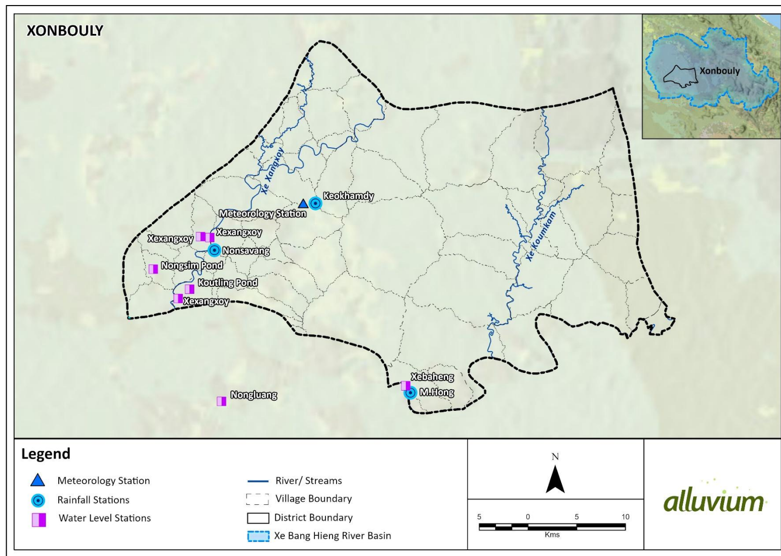
Figure 13. Meteorology and hydrology station in Xonbully District, Savannakhet Province
